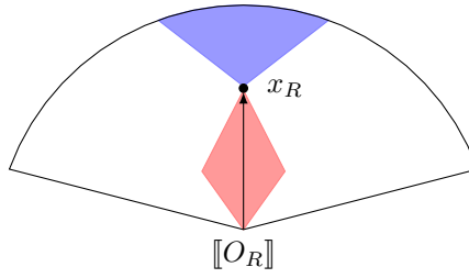
■ Figure 1 The encoding of O_R , of the future and of the past of a reversible process R .
